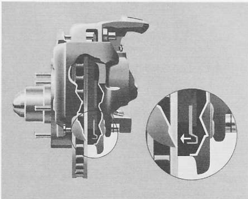
Front Disc Brake with Audible Wear Sensor
