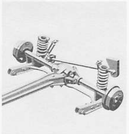
Torque Arm Rear Suspension
